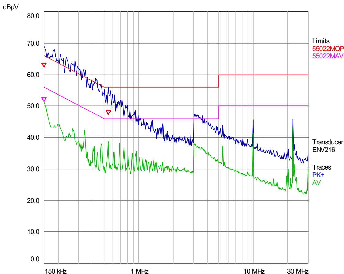
Figure 24. Conducted EMI
