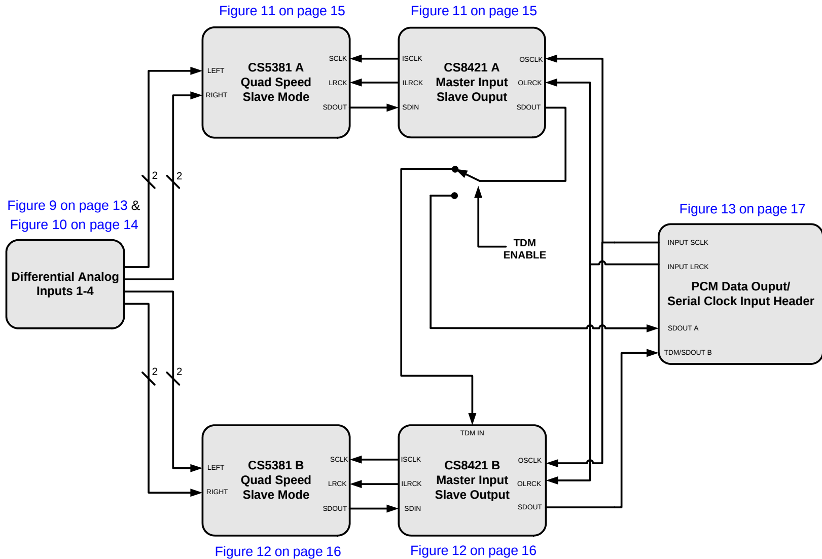
Figure 8. Block Diagram
