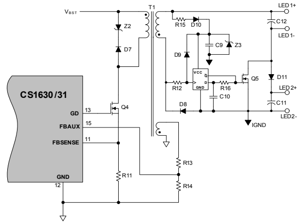
Figure 18. Flyback Series Output Model
