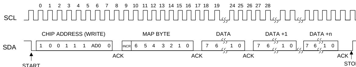
Figure 11. Control Port Timing, I²C Write
