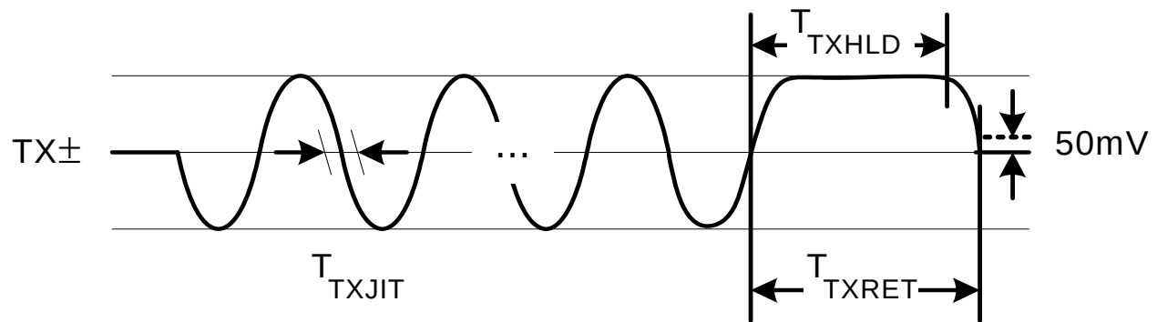
Figure 19. 10BASE-T Transmit
