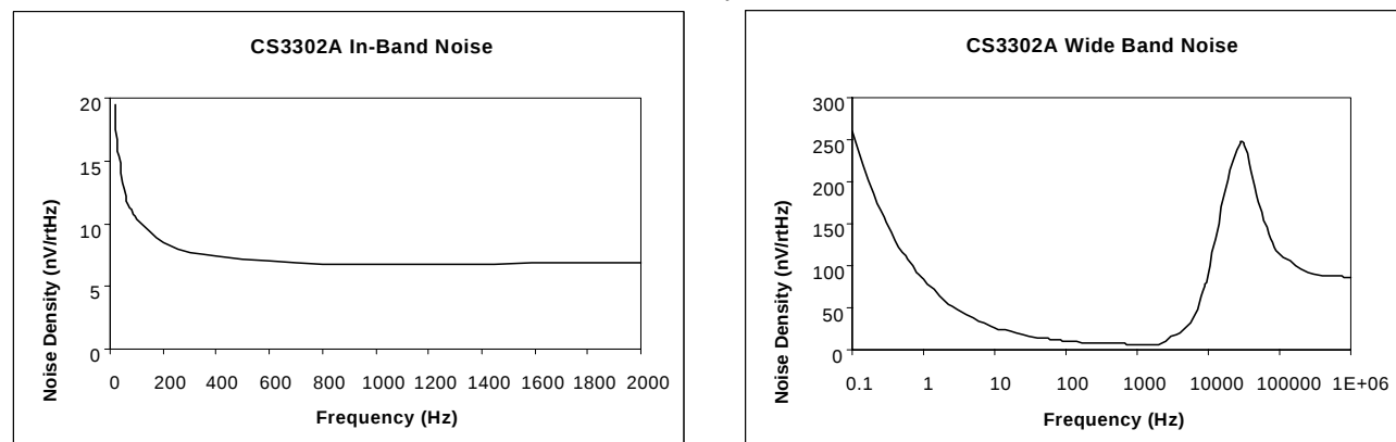
Figure 1. CS3302A Noise Performance
