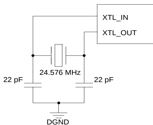
Figure 24. External Crystal
