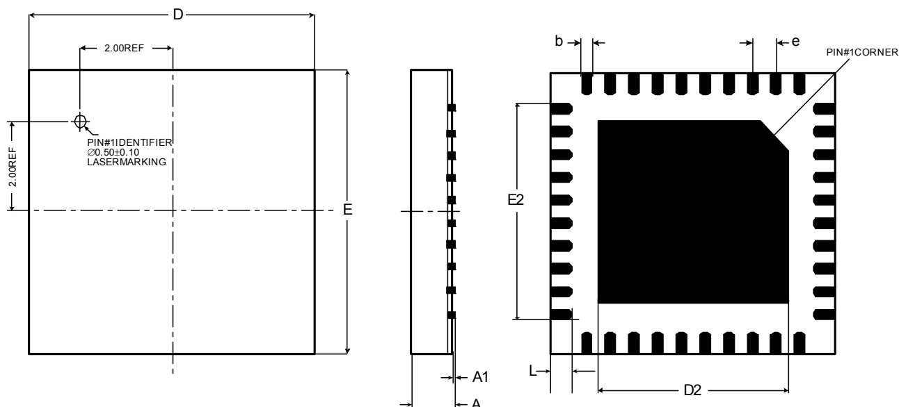
Figure 46. Package Drawing
