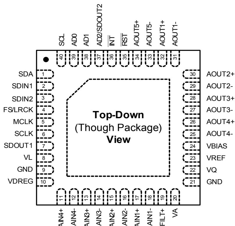
Figure 1. CS4234 Pinout
