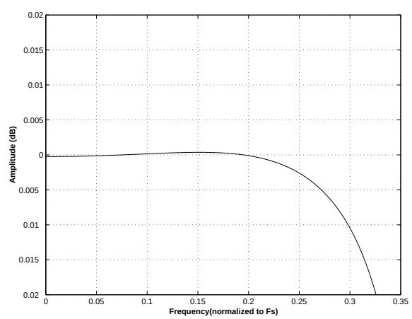
Figure 54. Double-Speed (slow) Passband Ripple
