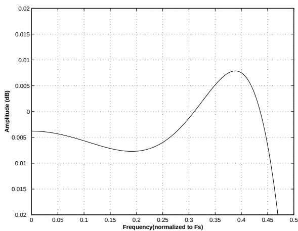
Figure 42. Single-Speed (fast) Passband Ripple
