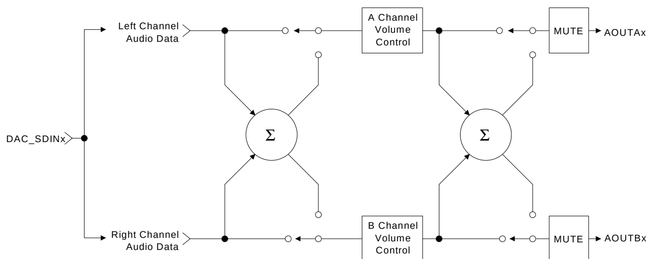
Figure 9. ATAPI Block Diagram (x = channel pair 1, 2, 3)
