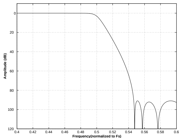
Figure 40. Single-Speed (fast) Transition Band
