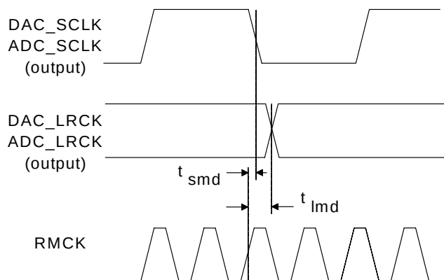
Figure 1. Serial Audio Port Master Mode Timing
