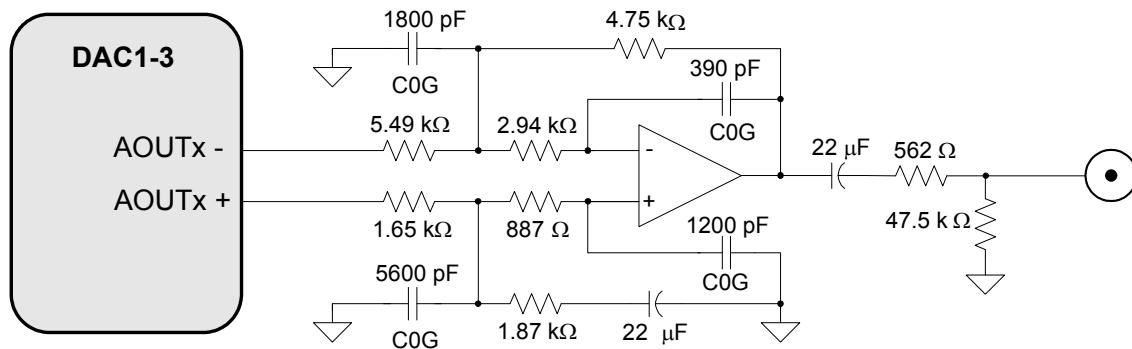
Figure 24. Active Analog Output Filter
