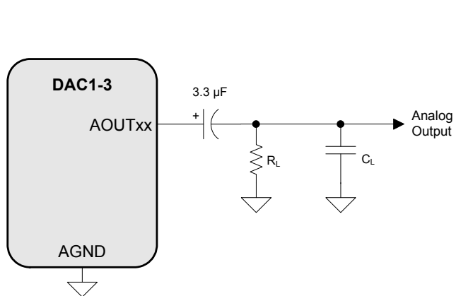
Figure 3. Output Test Load
