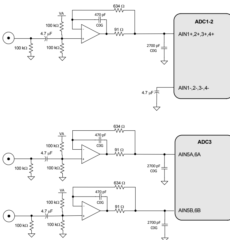
Figure 21. Single-Ended Active Input Filter
