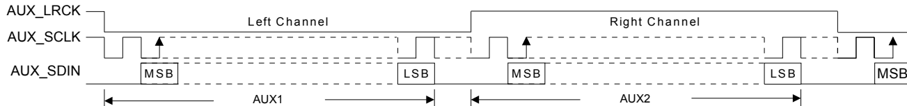
Figure 15. AUX I 2 S Format
