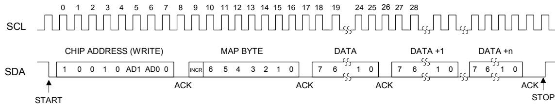
Figure 18. Control Port Timing, I²C Write
