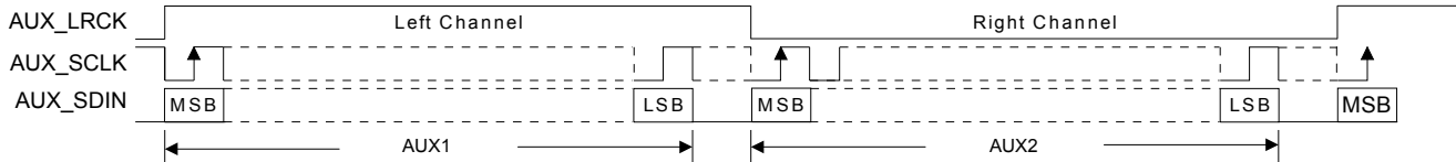
Figure 16. AUX Left-Justified Format
