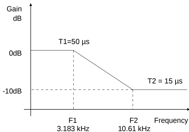
Figure 6. De-Emphasis Curve
