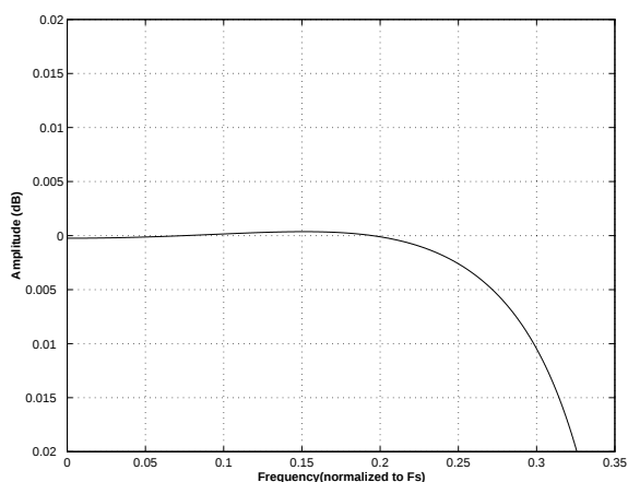
Figure 28. Double-Speed (slow) Passband Ripple
