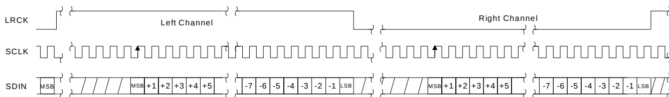
Figure 7. Right-Justified Data
