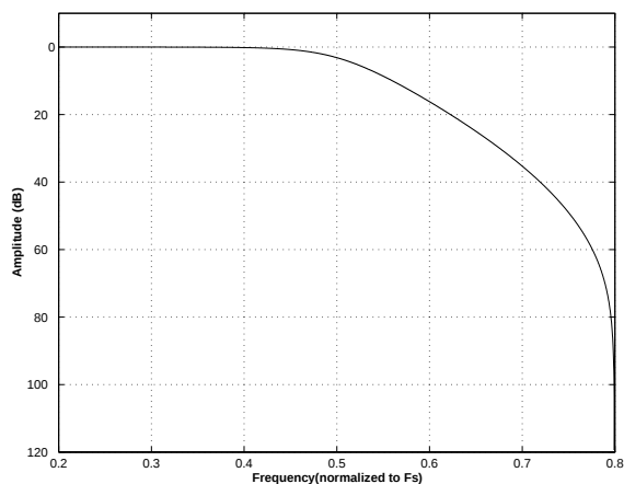
Figure 26. Double-Speed (slow) Transition Band
