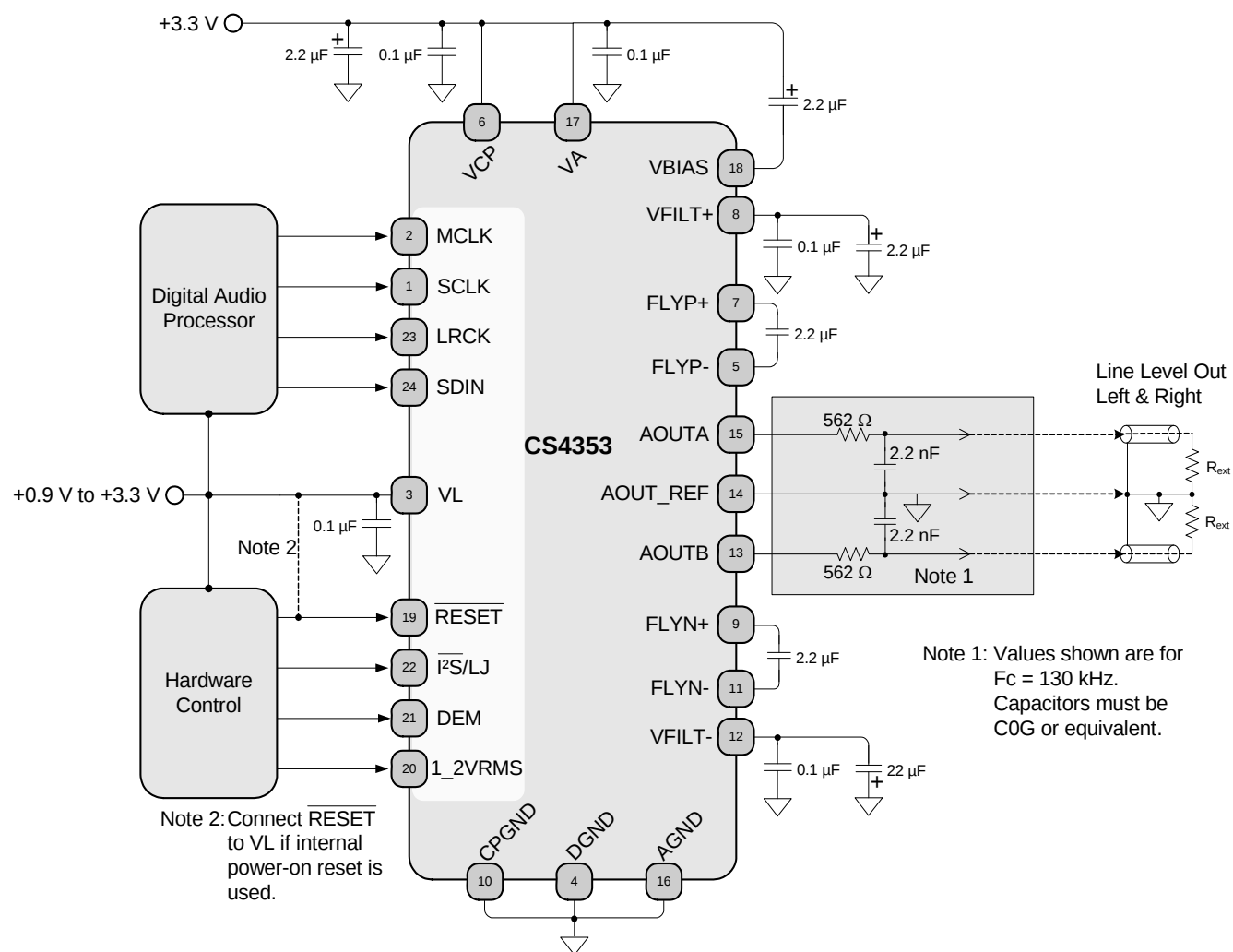
Figure 3. Typical Connection Diagram
