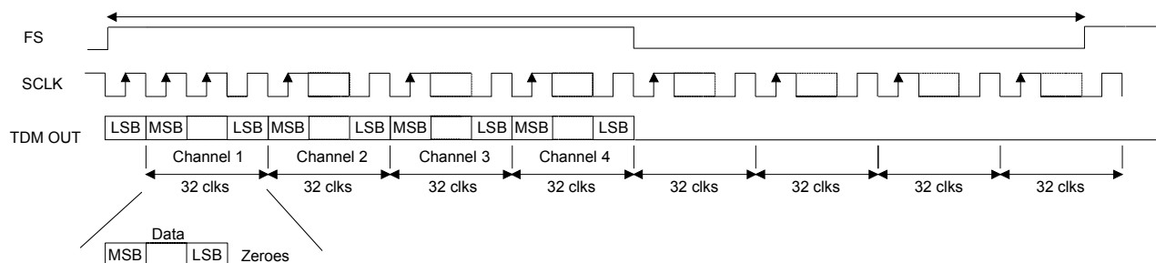
Figure 12. TDM Format
