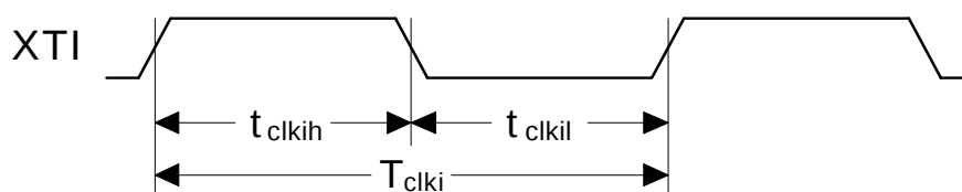
Figure 2. XTI Timing
