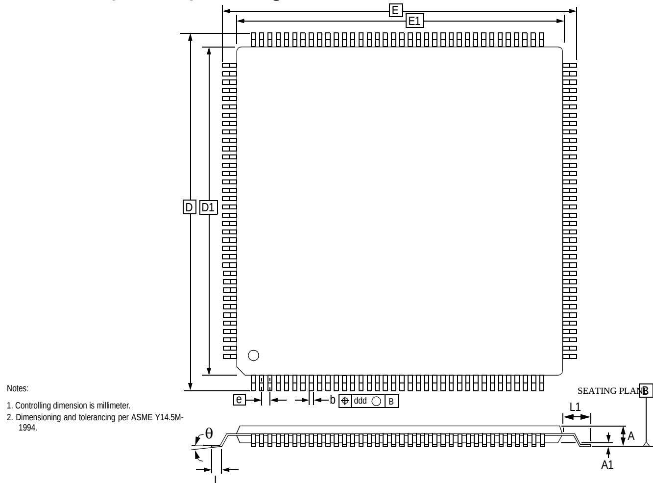
Figure 22. 144-Pin LQFP Package Drawing
