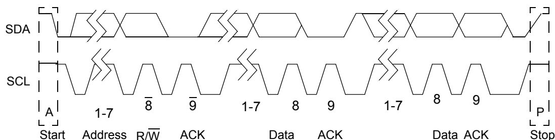
Figure 26. I 2 C Protocol
