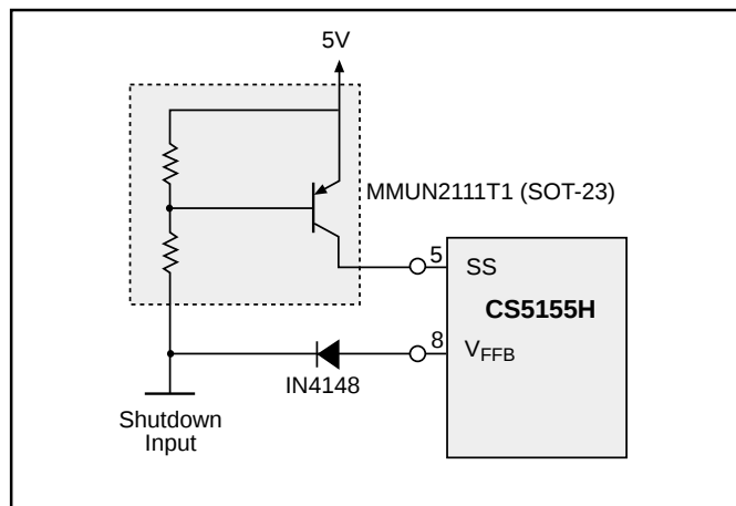
Figure 14: Implementing shutdown with the CS5155H.
