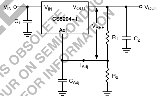
Figure 10. Resistor Divider Scheme for the Adjustable Version
