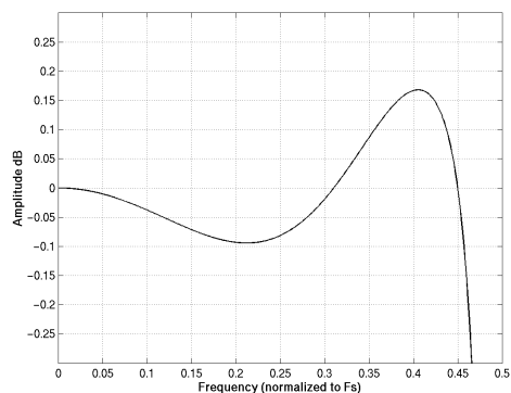
Figure 23. ADC Passband Ripple
