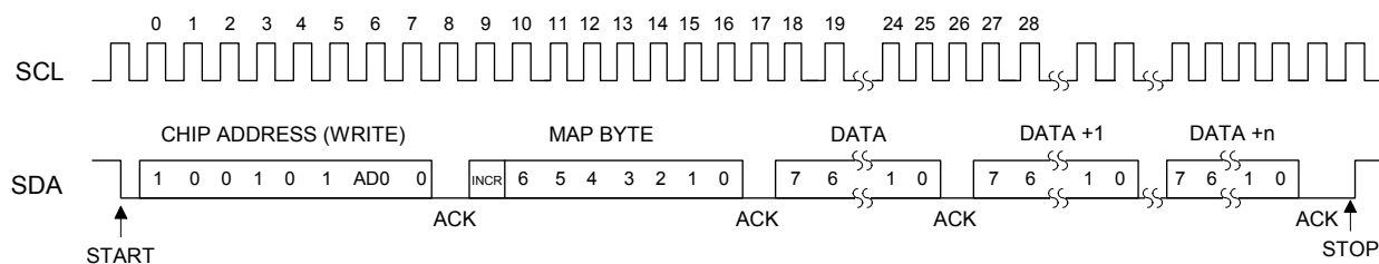
Figure 19. Control Port Timing, I²C Write
