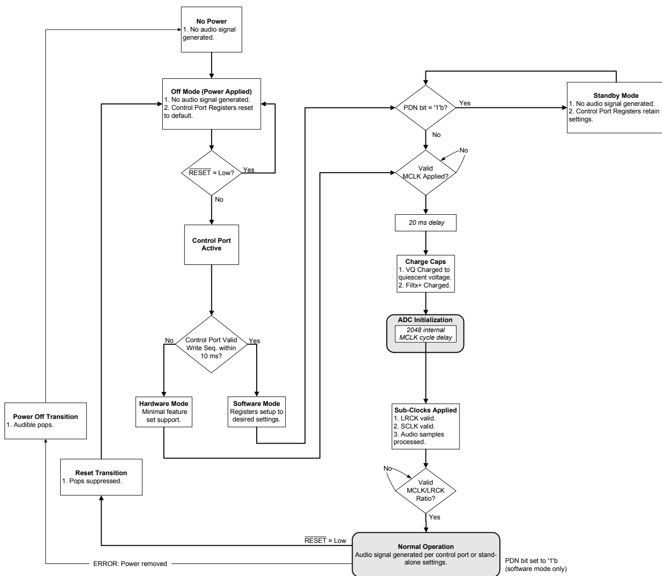
Figure 17. Initialization Flow Chart
