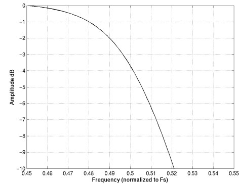
Figure 26. ADC Transition Band Detail
