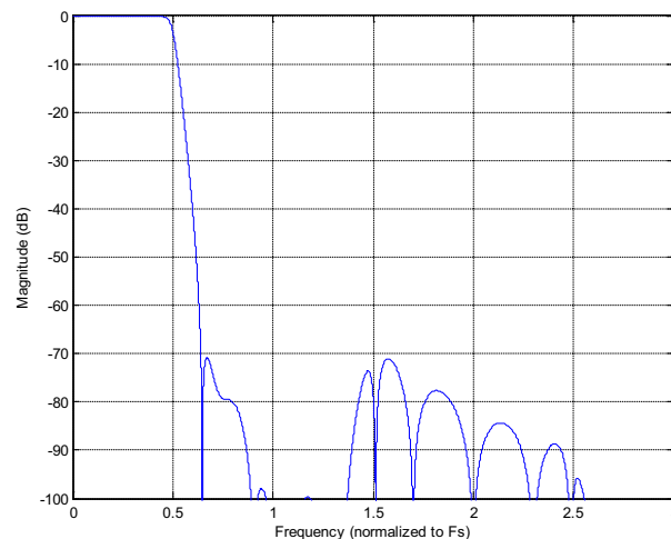
Figure 9-8. Stopband—ADCx, Notch Disabled
