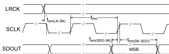
Serial Port Timing—Master Mode
