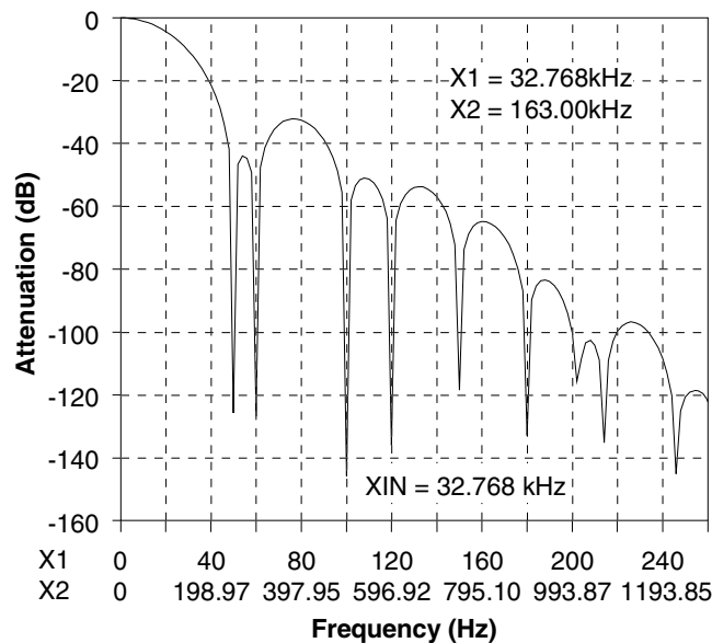
Figure 9. Filter Magnitude Plot to 260 Hz
