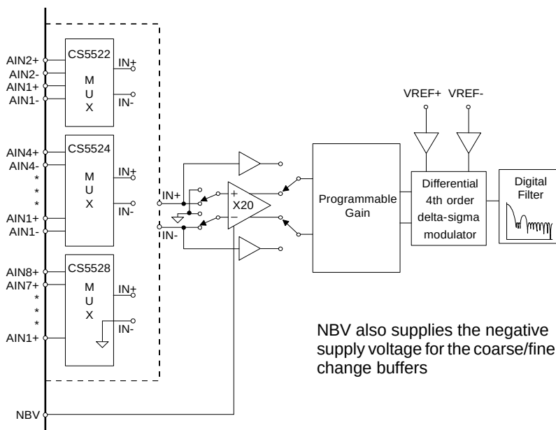
Figure 4. Multiplexer Configurations
