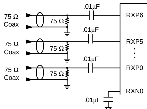
Figure 14. S/PDIF MUX Input Circuit
