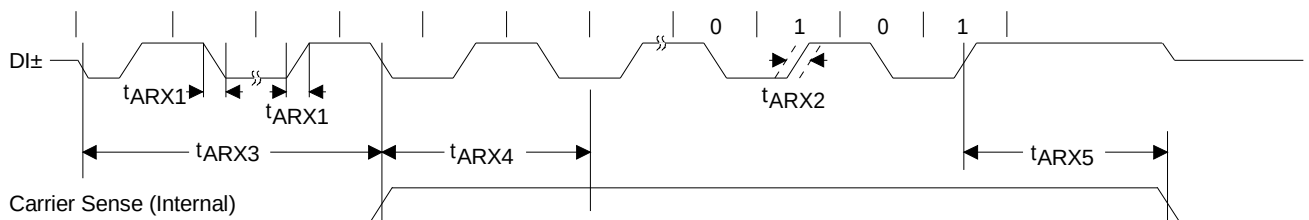
Figure 45. AUI Receive
