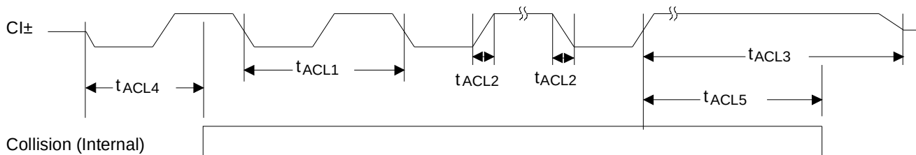
Figure 61. AUI Collision
