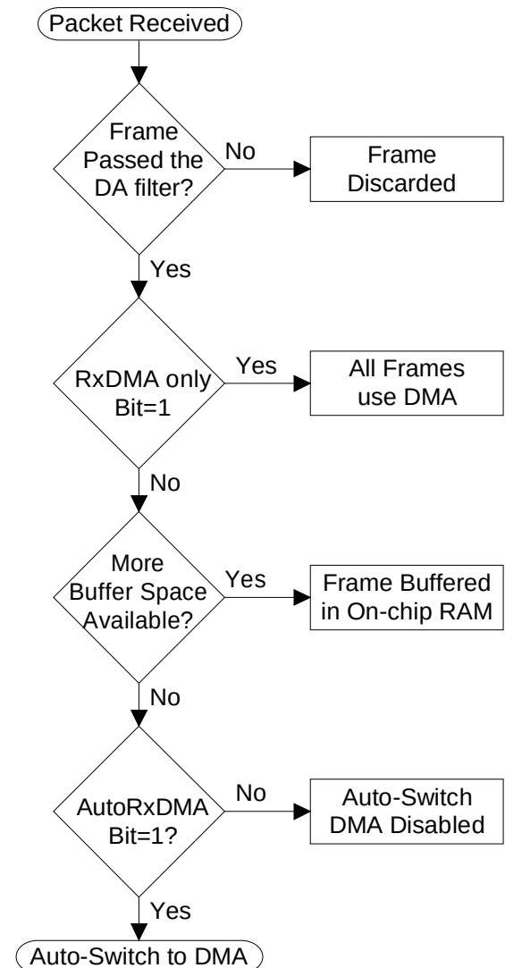
Figure 26. Conditions for Switching to DMA
