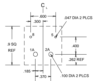
MOUNTING HOLE PATTERN TOP OF PCB
