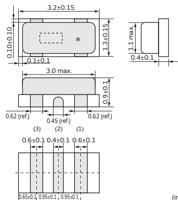
CSTCE_V 14.00-20.00MHz
