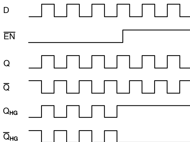
Timing Diagram
