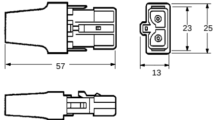
S3200-COCF2511
