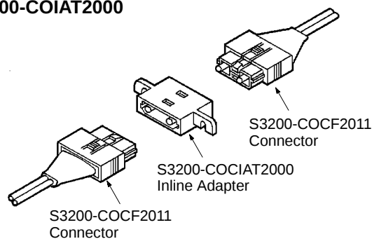
S3200-COIAT2000
