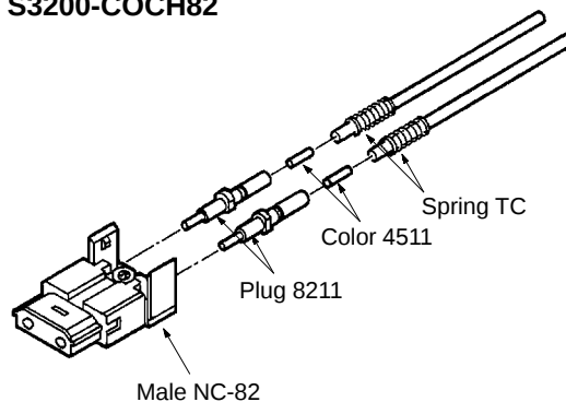
S3200-COCH82
