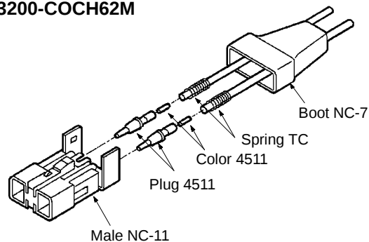
S3200-COCH62M
