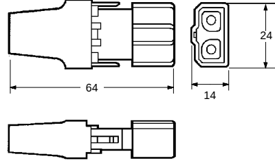
S3200-COCF2011
