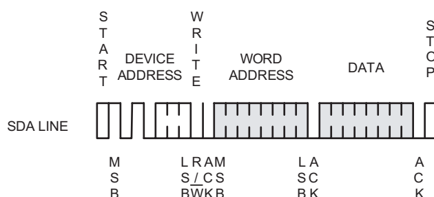
Figure 9. Byte Write
