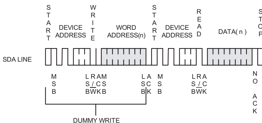
Figure 13. Random Read
