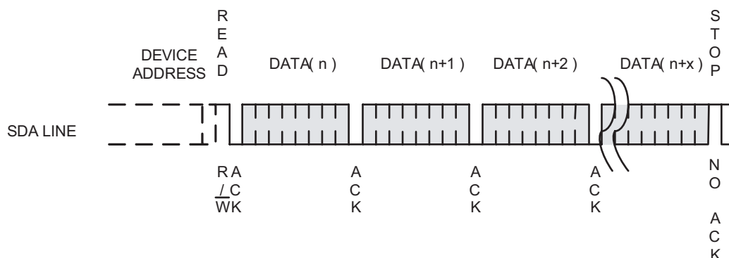
Figure 14. Sequential Read
