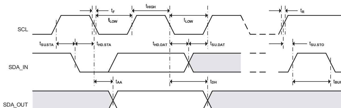
Figure 2. Bus Timing
