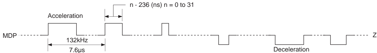
Timing Chart 1-7
