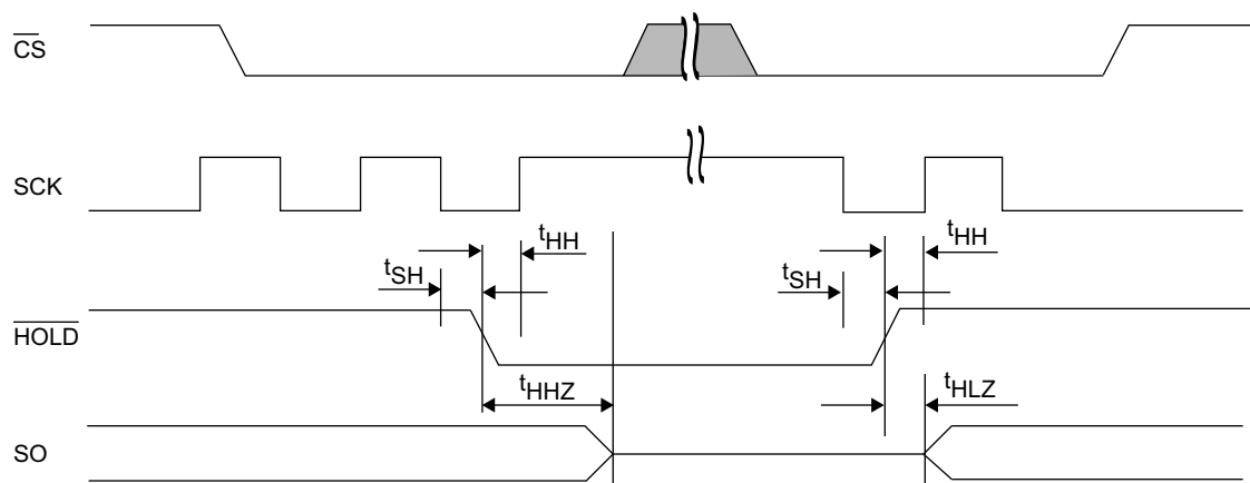
Figure 36. \overline{HOLD} Timing
