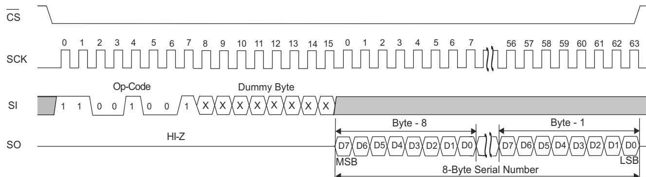
Figure 24. FAST_RDSN Instruction
