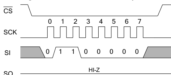
Figure 16. Software RECALL Operation
