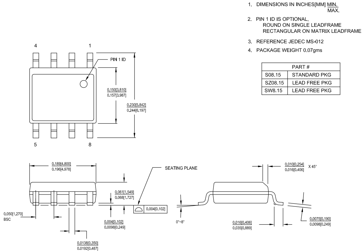
Figure 33. 8-pin SOIC (150 Mils) S0815/SZ815/SW815 Package Outline, 51-85066
