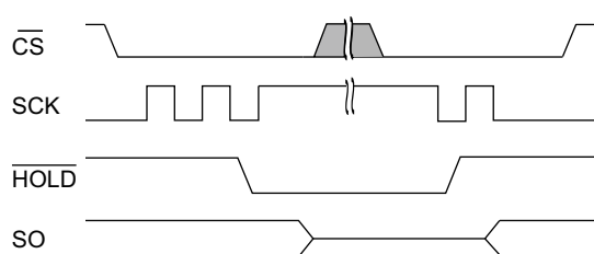
Figure 23. \overline{\text{HOLD}} Operation
