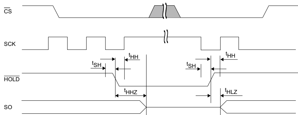
Figure 26. \overline{HOLD} Timing
