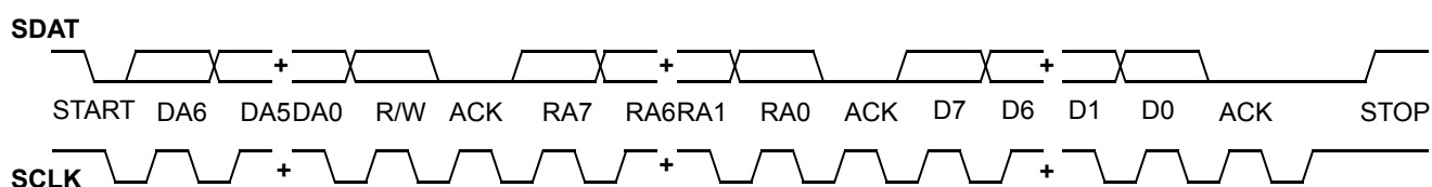
Figure 17. Definition for Timing on the Serial BUS
