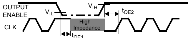
Figure 12. Output Enable and Disable Timing
