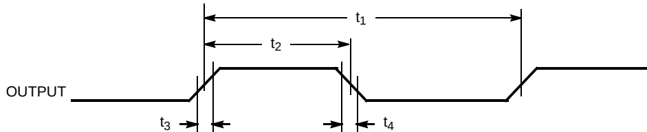
Figure 3. Output Three-State Timing [33]
