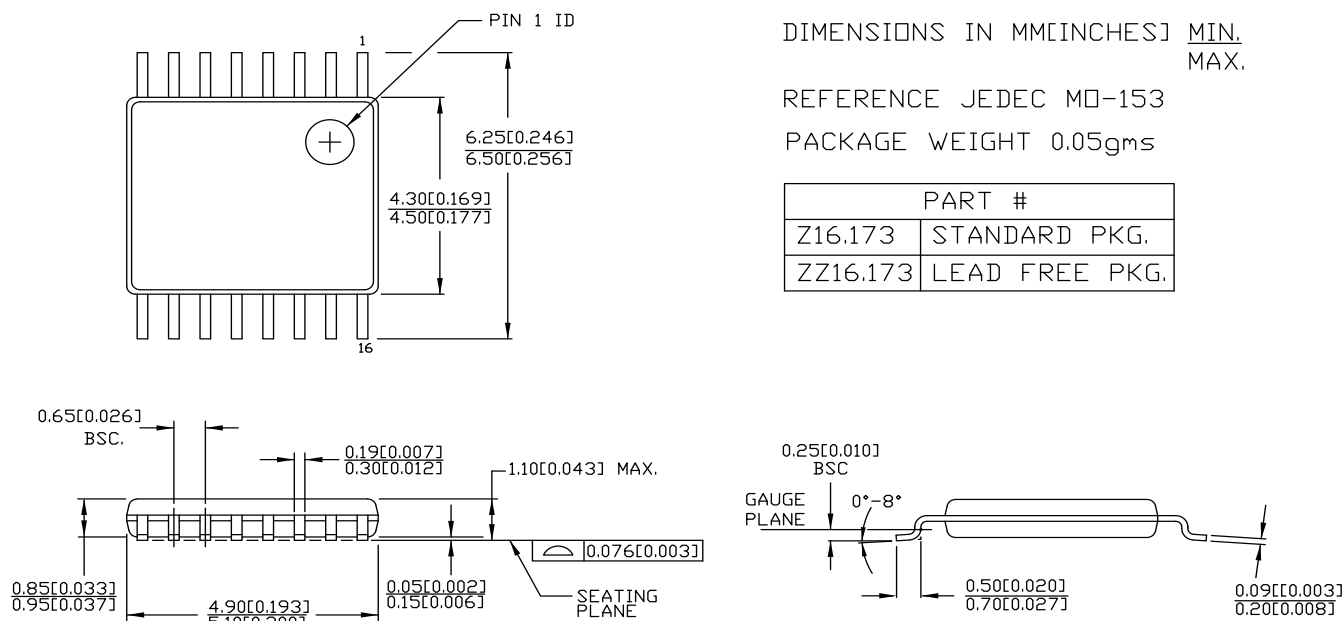
Figure 12. 16-pin TSSOP (4.40 mm Body) Z16.173/ZZ16.173 Package Outline, 51-85091
