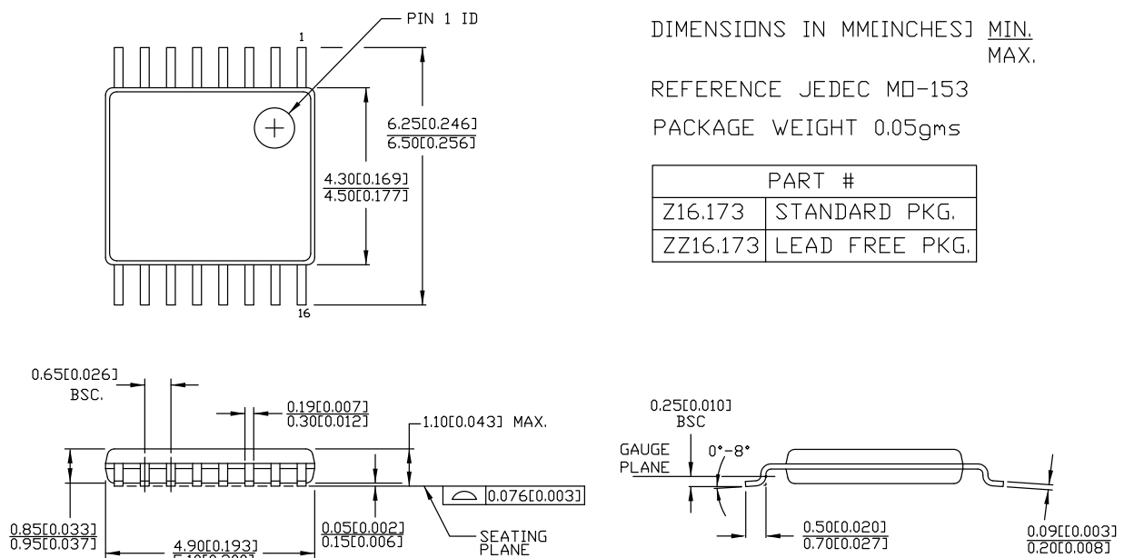
Figure 18. 16-pin TSSOP (4.40 mm Body) Z16.173/ZZ16.173 Package Outline, 51-85091
