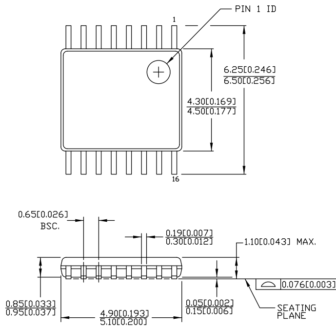
Figure 14. 16-pin TSSOP (4.40 mm Body) Z16.173/ZZ16.173 Package Outline, 51-85091
