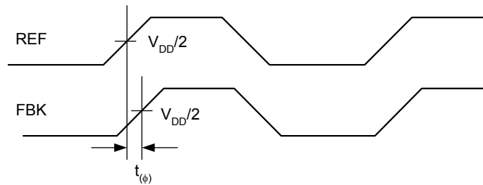
Figure 13. Phase Offset
