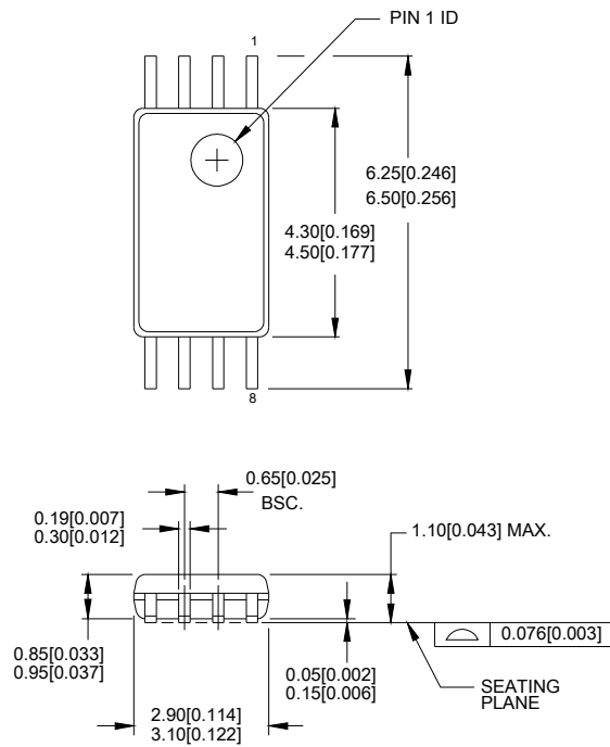
Figure 6. 8-Pin Thin Shrunk Small Outline Package (4.40 MM Body) Z8
