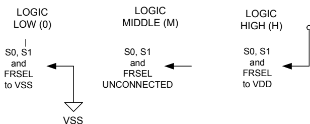
Figure 2. 3-Level Logic
