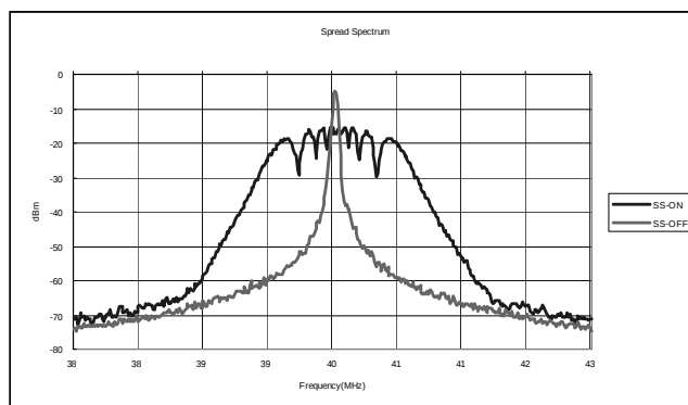
Figure 2. Spread Spectrum
