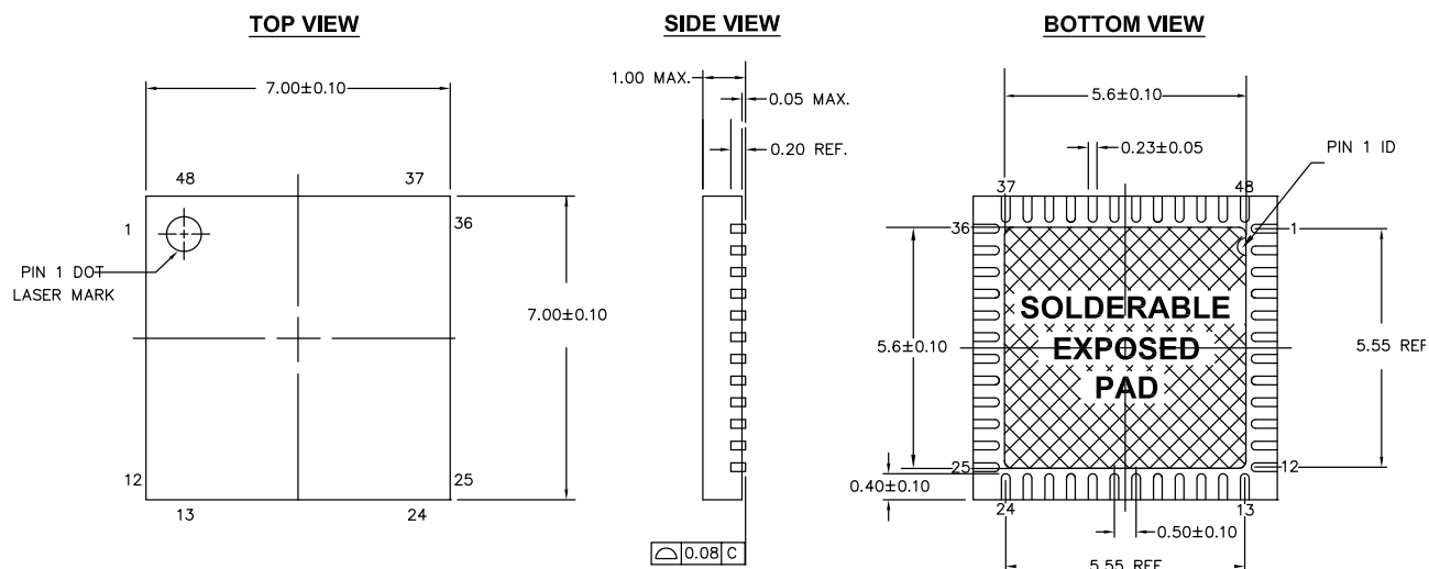
Figure 41. 48-Pin QFN (7 × 7 × 1.00 mm) LT48D 5.5 x 5.5 EPAD (Sawn) Package Outline
