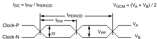
Figure 30. Differential Input Definitions
