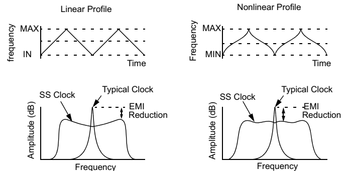
Figure 16. Spread-Spectrum Profile
