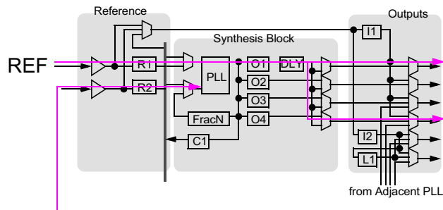
Figure 10. ZDB Configuration
