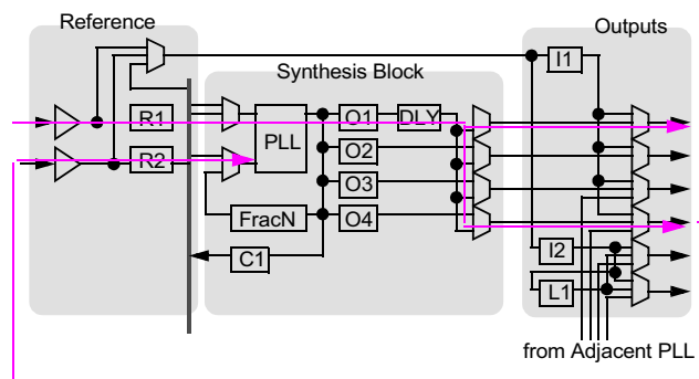
Figure 12. Early/Late Phase in ZDB Configuration
