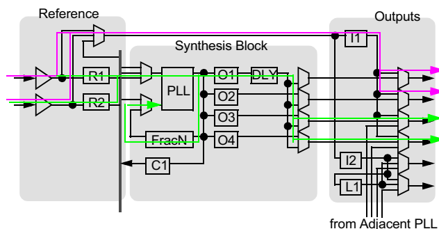
Figure 14. Clock Generator and NZDB
