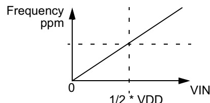
Figure 17. VCFS Profile
