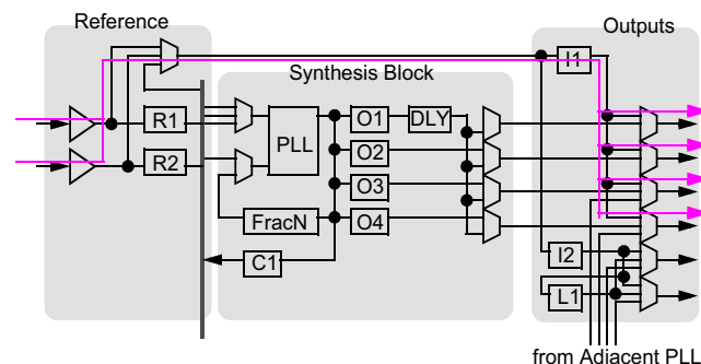
Figure 13. NZDB Configuration
