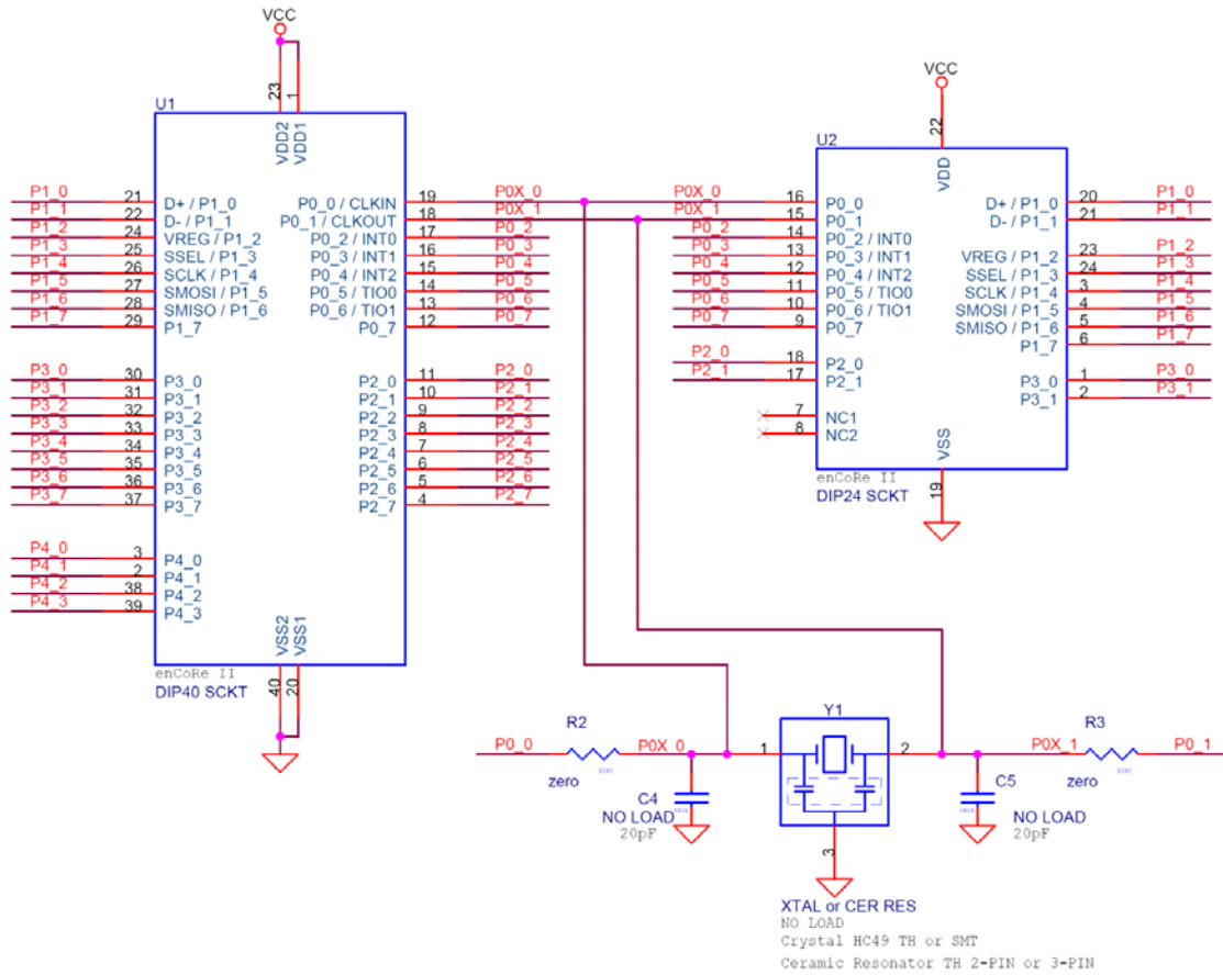
Figure 4-5. Schematic View of 24-Pin and 40-Pin DIP Sockets
