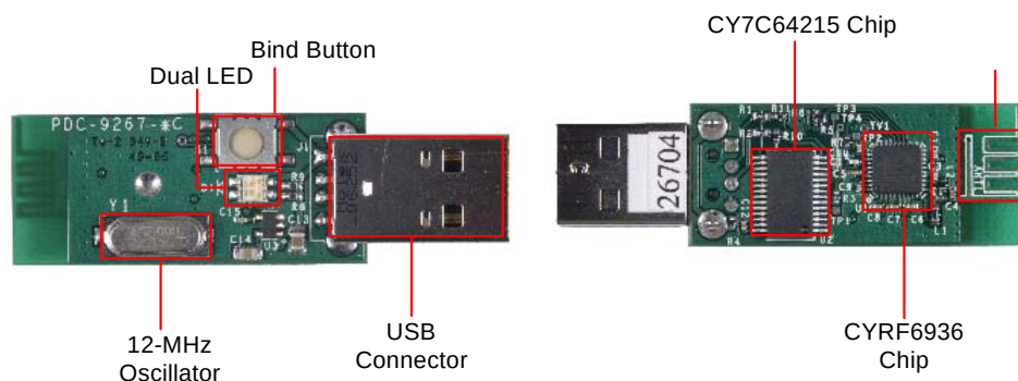
Figure 4-2. Bridge Board Functional Blocks
