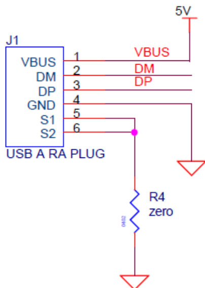
Figure 4-5. Schematic View of USB A Connector
