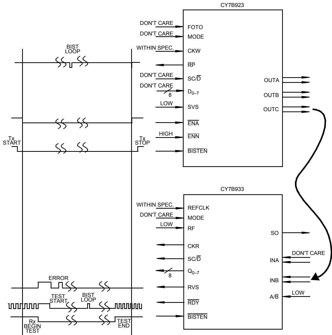
Figure 6. BIST Illustration
