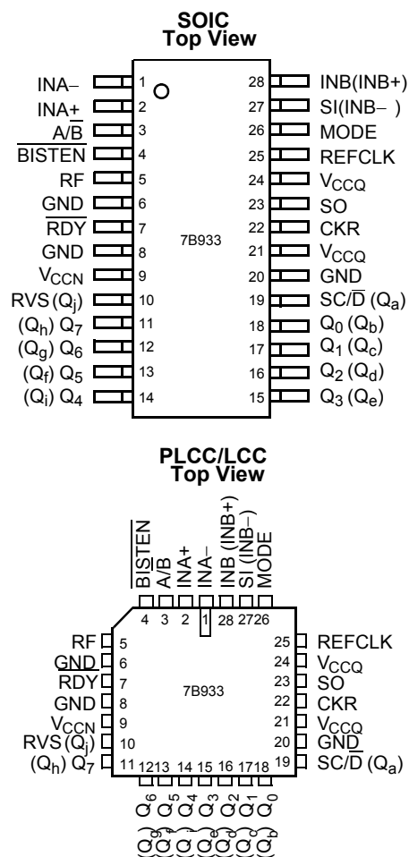
Figure 3. CY7B933 Receiver Pin Configurations
