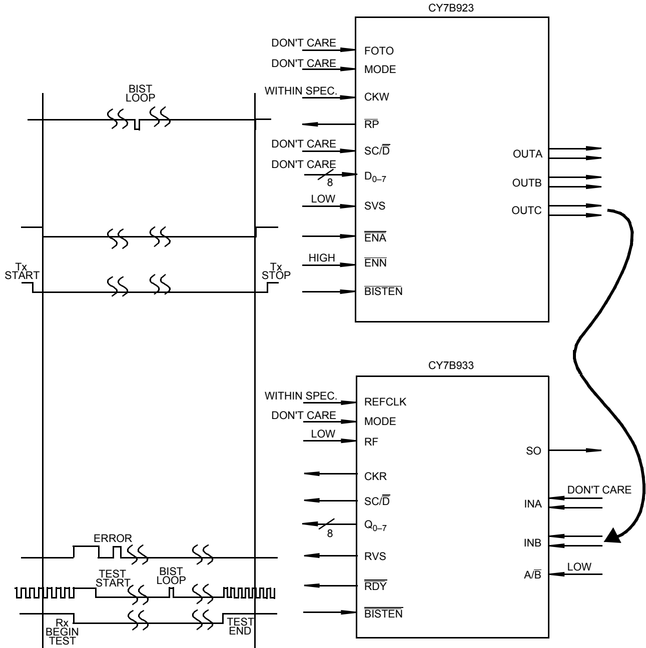
Figure 8. BIST Illustration
