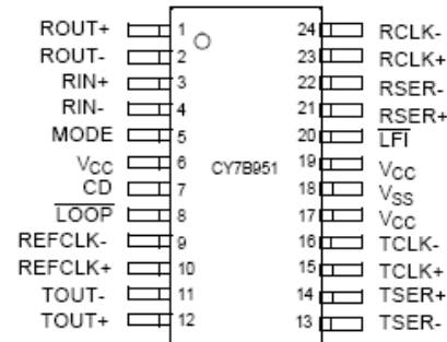
Figure 1. 24-pin SOIC (Top View)
